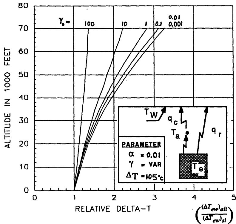
Figure 3-21: Effects of convection balance factor, \gamma , on the changes of \left(\frac{(\Delta T_{ew})_{alt}}{(\Delta T_{ew})_{sl}}\right) with altitude in a system with radiation factor \alpha=0.01
