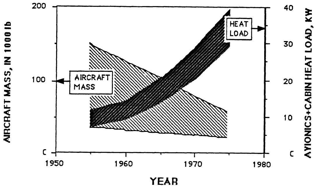
Figure 2-2: Trends in cabin and avionics heat load and aircraft mass [14].
