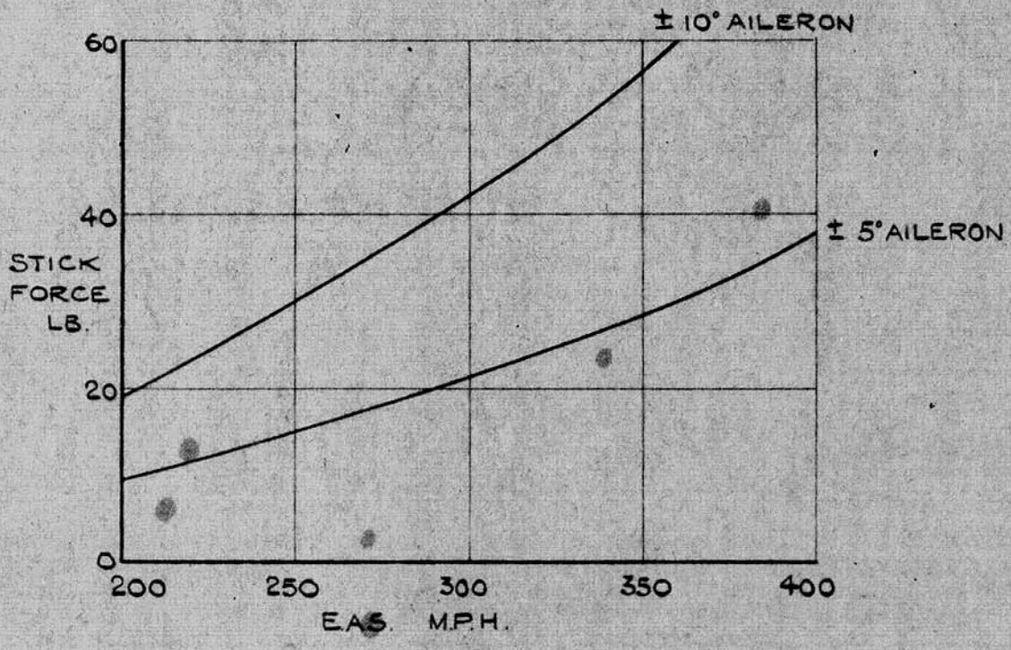
VARIATION OF STICK FORCE WITH SPEED & AILERON ANGLE F.W. 190
