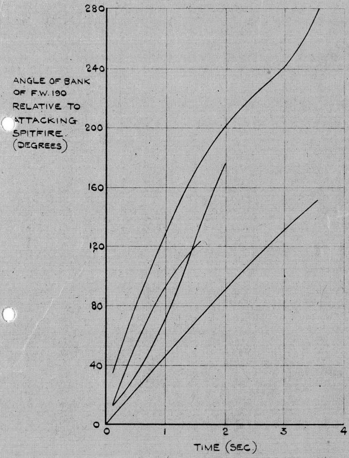
TIMES TO BANK ~ FROM COMBAT FILMS F.W. 190
