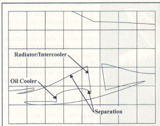
Figure 6 - Calculated boundary layer separation in the Mustang cooling system
