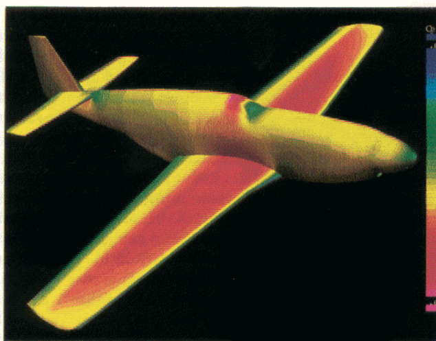
Figure 3 - Pressure distribution calculated on the P-51B Mustang.
