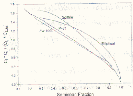
Figure 2 - Calculated wing loading comparison with the aircraft trimmed at 360 kt and 15,000 feet altitude to representative gross weights and CG locations.
