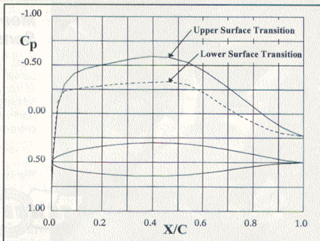
Figure 5 - Calculated Mustang wing airfoil pressure distribution and boundary layer transition locations in cruise, for ideal surface conditions.
