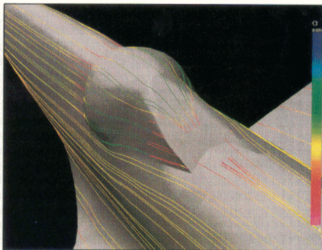
Figure 8 - Calculated Spitfire windshield boundary layer separation. Separation is calculated to take place at the base of the windshield where the streamline traces end. The location where the separated flow is estimated to reattach higher up the windshield is shown by where the streamline traces resume.
