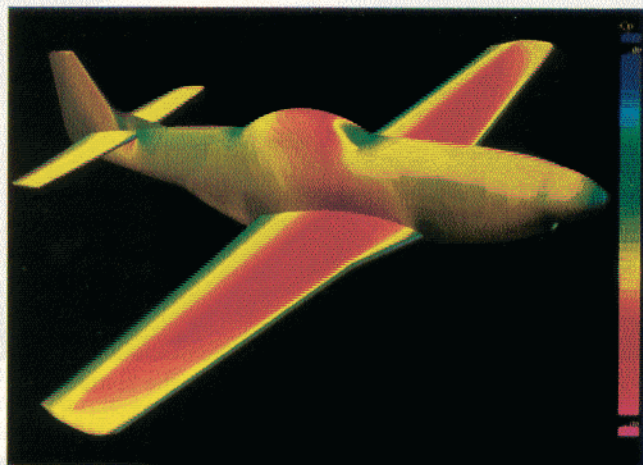
Figure 4 - Pressure distribution calculated on the P-51D Mustang.
