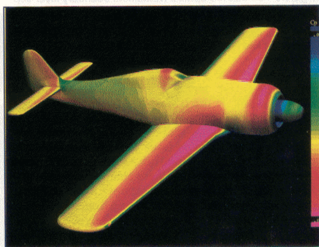
Figure 10 - Pressure distribution calculated on the Fw 190 A-8.
