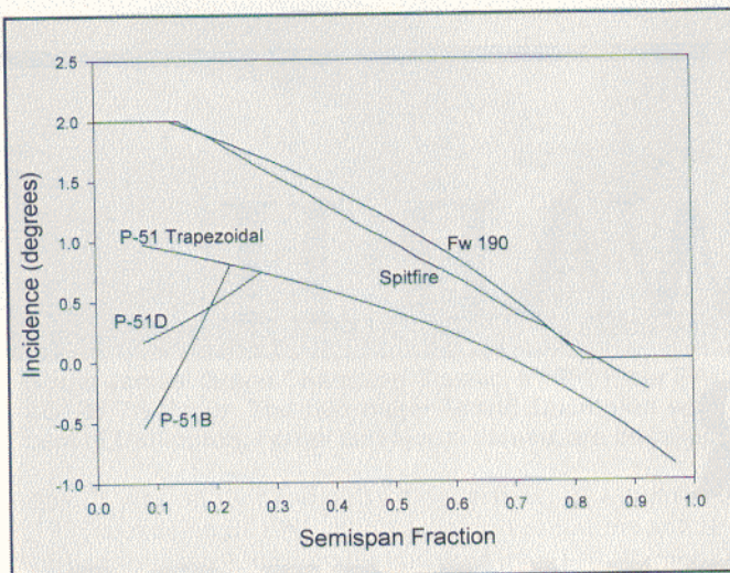
Figure 1- Wing twist distributions for the P-51B, P-51D, Spitfire and Fw 190.
