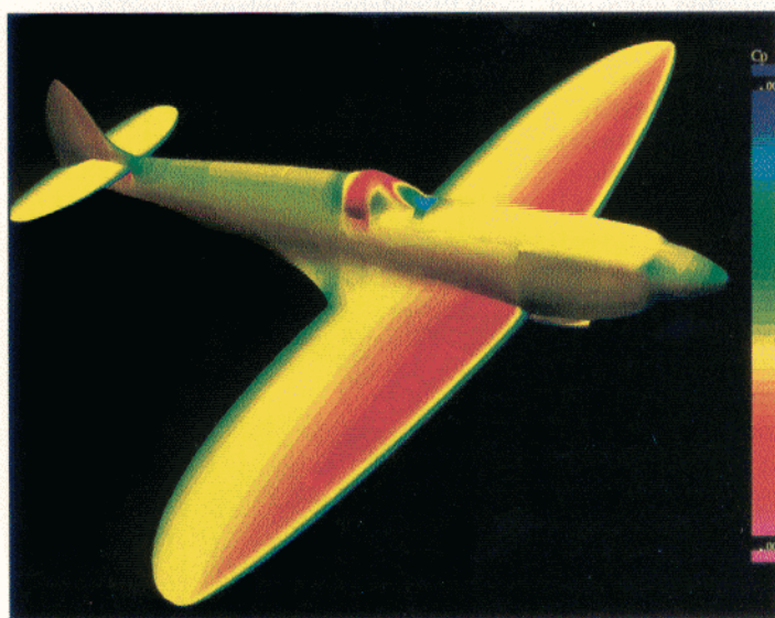
Figure 7 - Pressure distribution calculated on the Spitfire IX.
