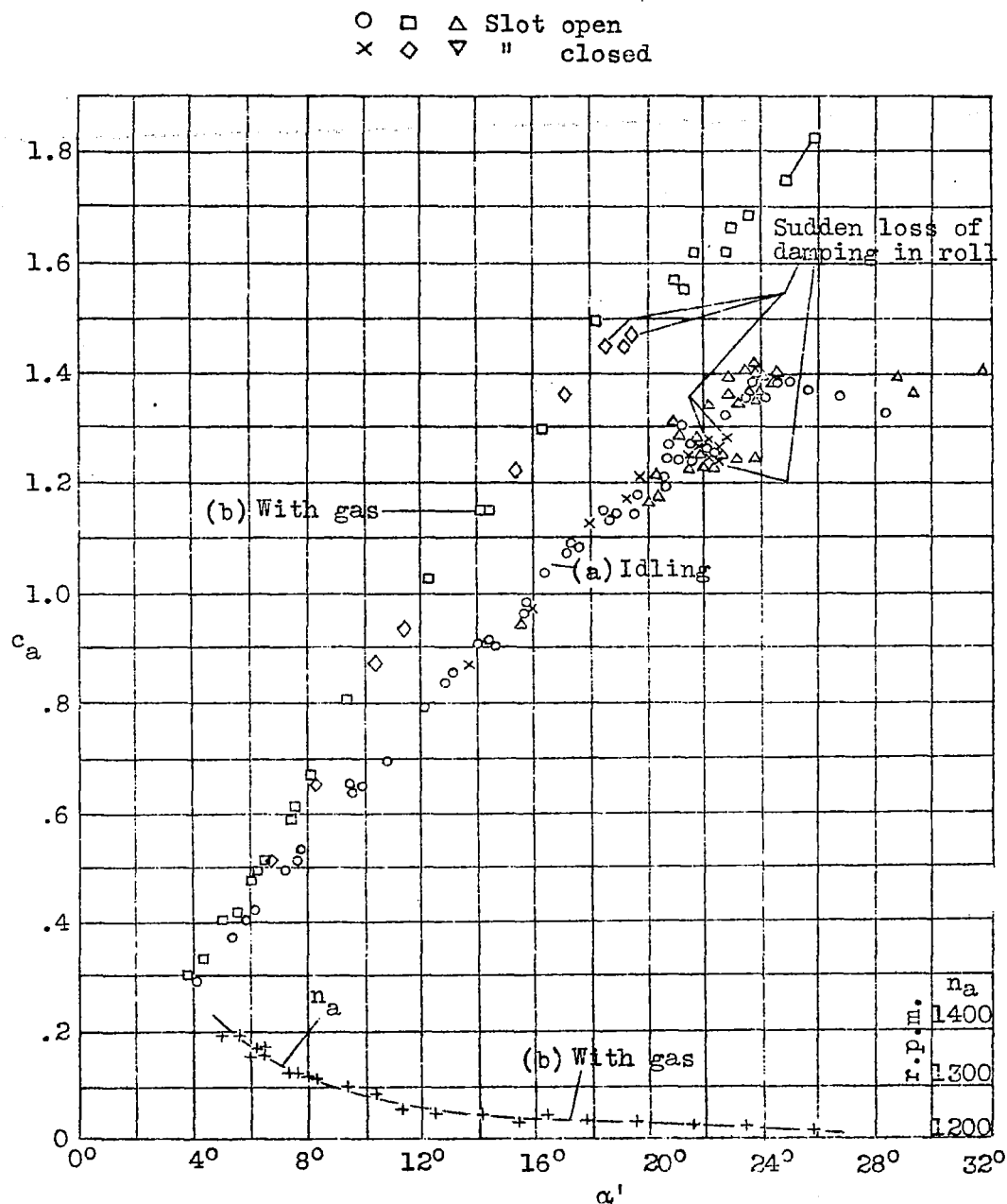
Fig.6 Lift coefficient c_a versus reference angle \alpha' in throttle flight (a) and with certain throttle setting (b).
