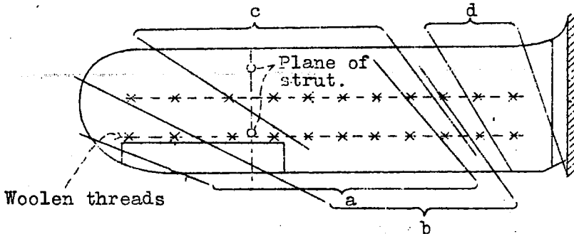
Fig. 8A Threads rigged up on top side of lower wing, and section of picture of series a. to d.
