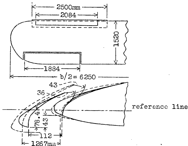
Fig. 2 Position and mounting of Handley-Page automatic control-slot at upper wing. The dotted lines denote the examined new type of slot.
