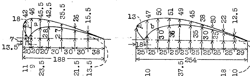
Fig. 3 Dimensions of old (a) and new (b) type of slot.
