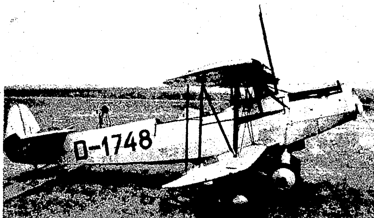
Fig. 4a Albatros L 75 with slots. Note the streamline tanks (Fig. 4b) suspended from the lower wing. One tank serves for dropping ballast weight [28.5 liters (7.53 gal.) of water].
