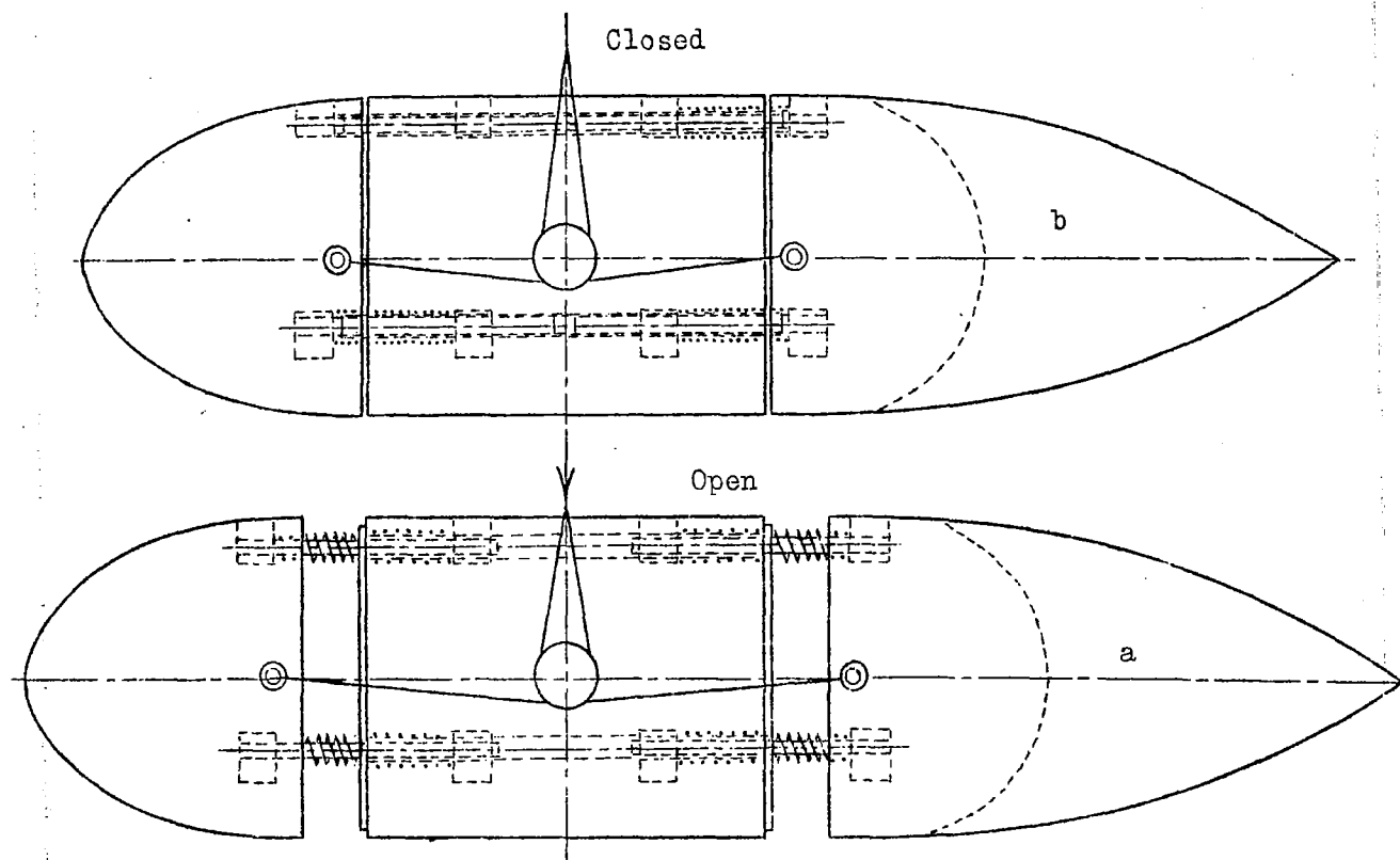
Fig. 4b Sketch of wing tanks, (a) open and (b) closed. The tank is closed from the observers seat by mechanical-cable device and ratchet. Upon release of ratchet, pressure springs tensed on the inside, effect sudden opening of tank. The openings are large enough to assure quick emptying of water.
