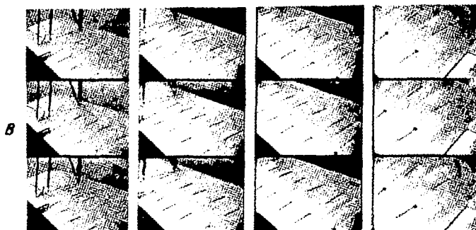
Fig. 8B Behavior of threads in normal flight. The equilibrium position corresponds to c_a \sim 0.65 ( \alpha' \sim 5^\circ ). Insignificant separation at wing root (film series d).
