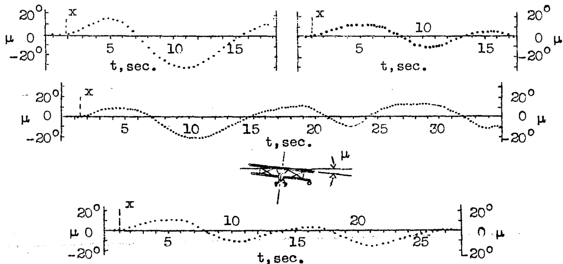
Fig. 12 Time rate of \mu for airplane, slots open, after initiation of motion in roll and subsequent sideslip. x denotes the start of water release.
