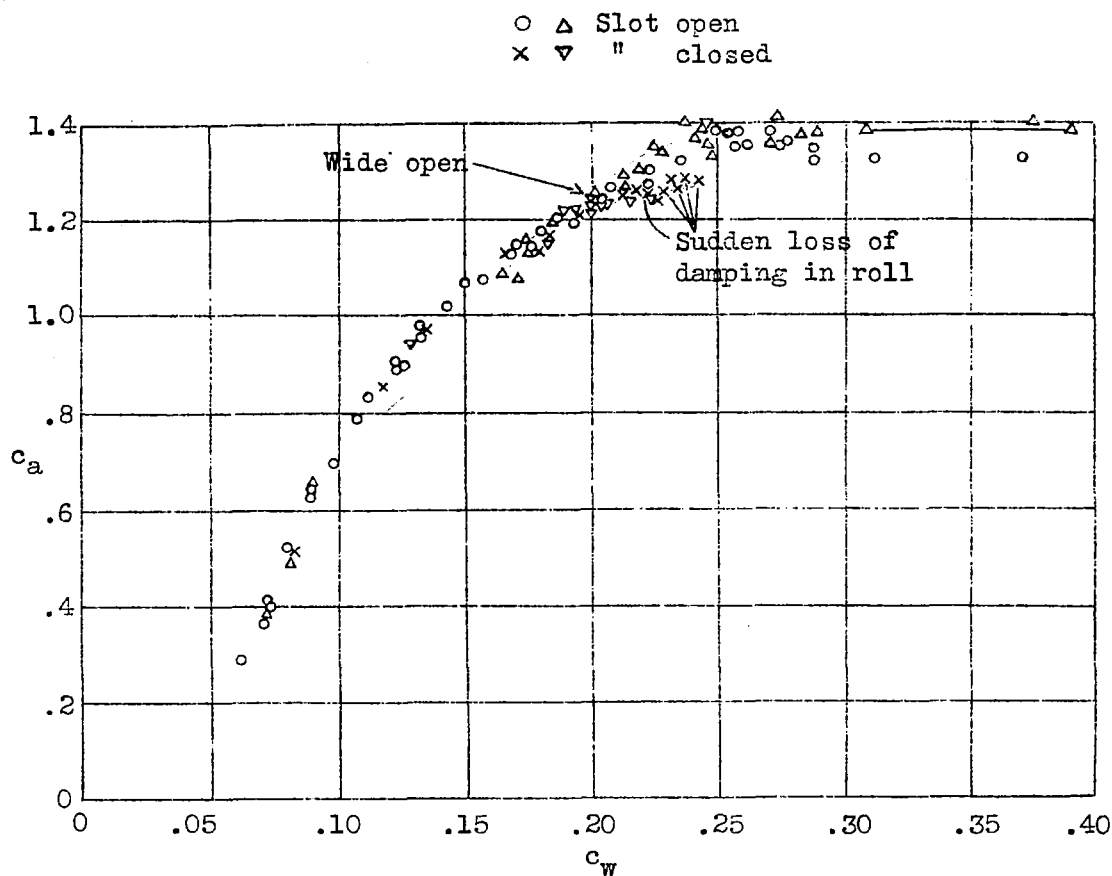
Fig.5 Gliding polar curves (throttle flight) with open and locked slots. The test point of those polars, denoted by \Delta and \nabla correspond to the different initial equilibrium positions immediately preceding the applied motion in roll.
