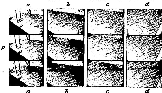
Fig. 8 Cinematograph pictures (speed 12-14 m/sec.) of the action of the woolen threads at different flight attitudes with certain throttle setting.
