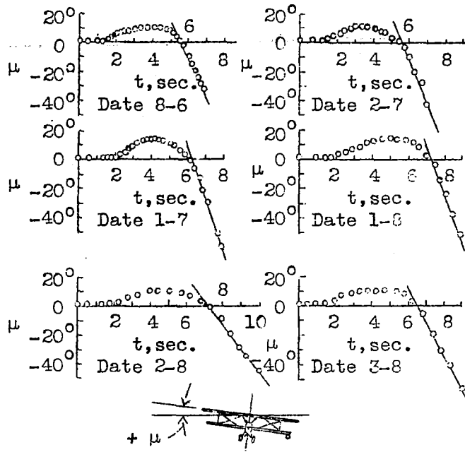
Fig. 11 Time rate of \mu for airplane, control slots locked, after initiation of motion in roll and subsequent sideslip.
