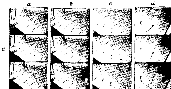
Fig. 8C Behavior of threads shortly before reaching maximum lift. The equilibrium position corresponds to c_a \sim 1.15 ( \alpha' \sim 12^\circ ). The separation is more pronounced, starting at the wing root and advancing to the plane of strut (film series b, c and d).
