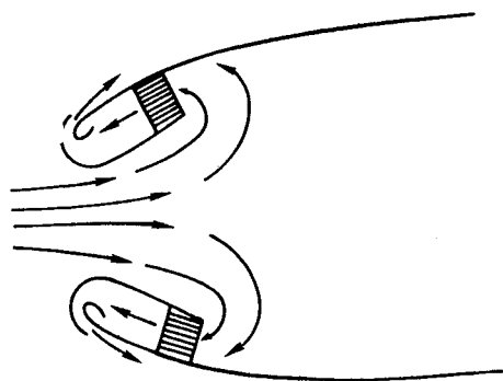
Fig. 11 Nose slot exit in asymmetric inlet cowl.
