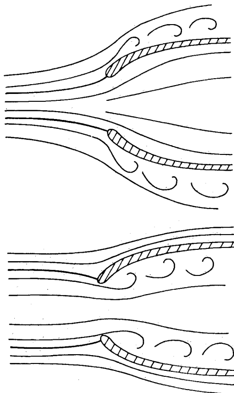
Fig. 4 Effect of stagnation point location on inlet separation.
