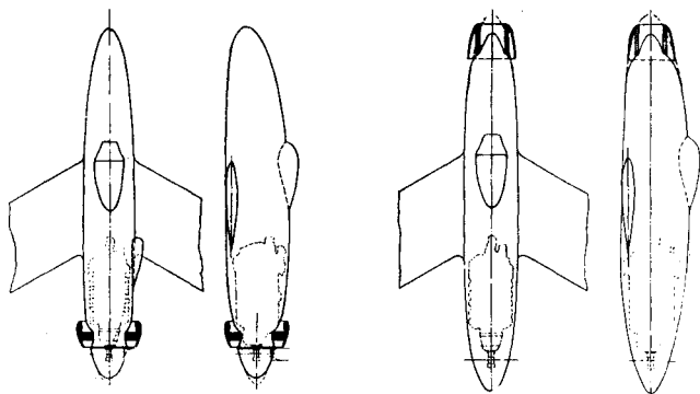
Fig. 16 Fore and aft ring radiator installations from Ref. 2.
