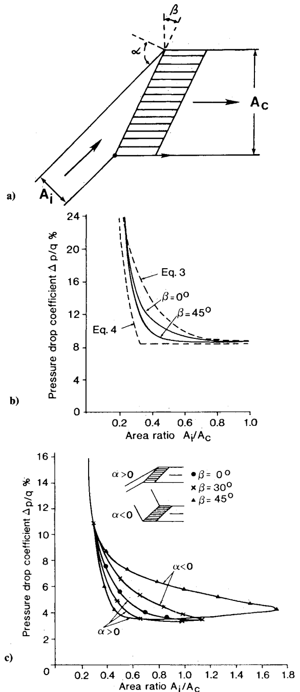
Fig. 10 Effects of staggered radiator on oblique flow: a) flow model, b) results from Ref. 2, and c) further results from Ref. 2.
