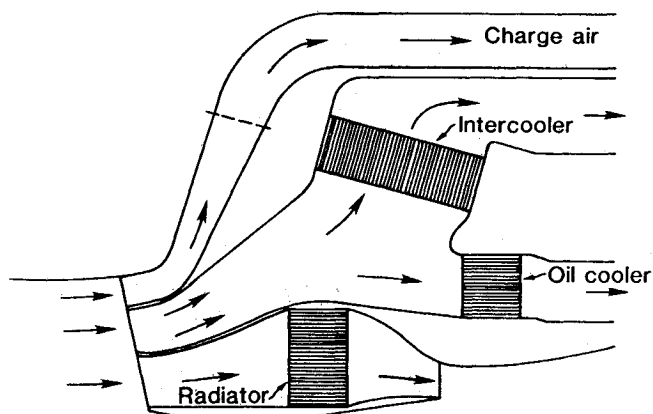
Fig. 2 Representative liquid-cooled aircraft engine cooling installation.
