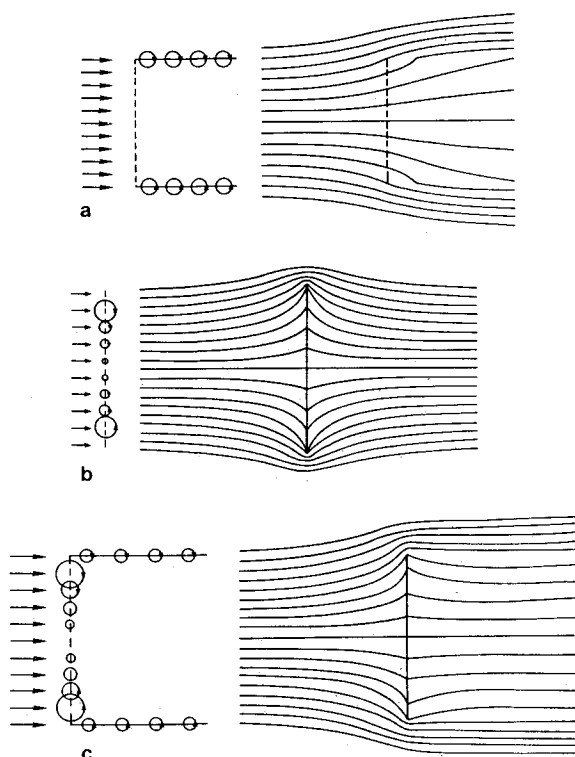
Fig. 7 Singularity models for development of streamline diffusers: a) vortices on bounding streamtube, b) vortices on radiator disk, and c) combined streamtube and radiator vortices.
