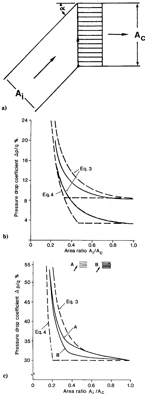
Fig. 9 Oblique flow effects: a) flow model, b) results from Ref. 2, and c) results from Ref. 15.
