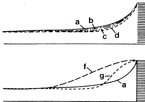
Fig. 8 Comparison of diffuser shapes listed in Table 1.
