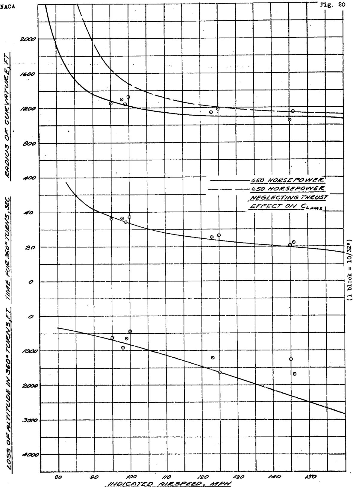
FIGURE 20.- CALCULATED AND EXPERIMENTAL DETERMINATIONS OF THE TURNING PERFORMANCE, IN STEADY TURNS, AT 27000 FEET ALTITUDE, MAXIMUM LIFT COEFFICIENT, FLAPS 22° DOWN OF A NAVY F2A-3 AIRPLANE.
