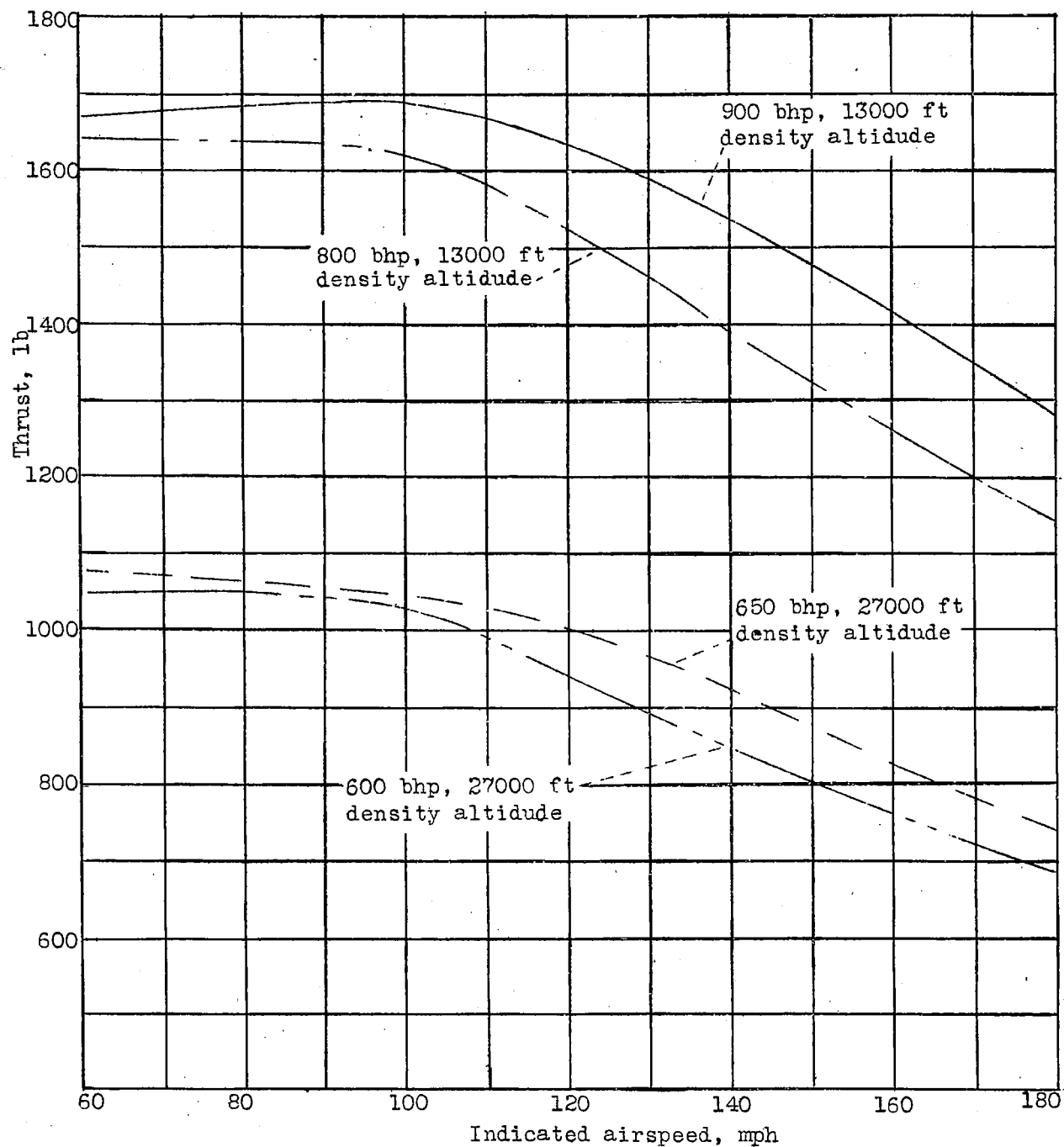
Figure 13.- Variation of thrust with indicated airspeed for various altitudes and horsepower at 2300 rpm, Navy F2A-3 airplane.
