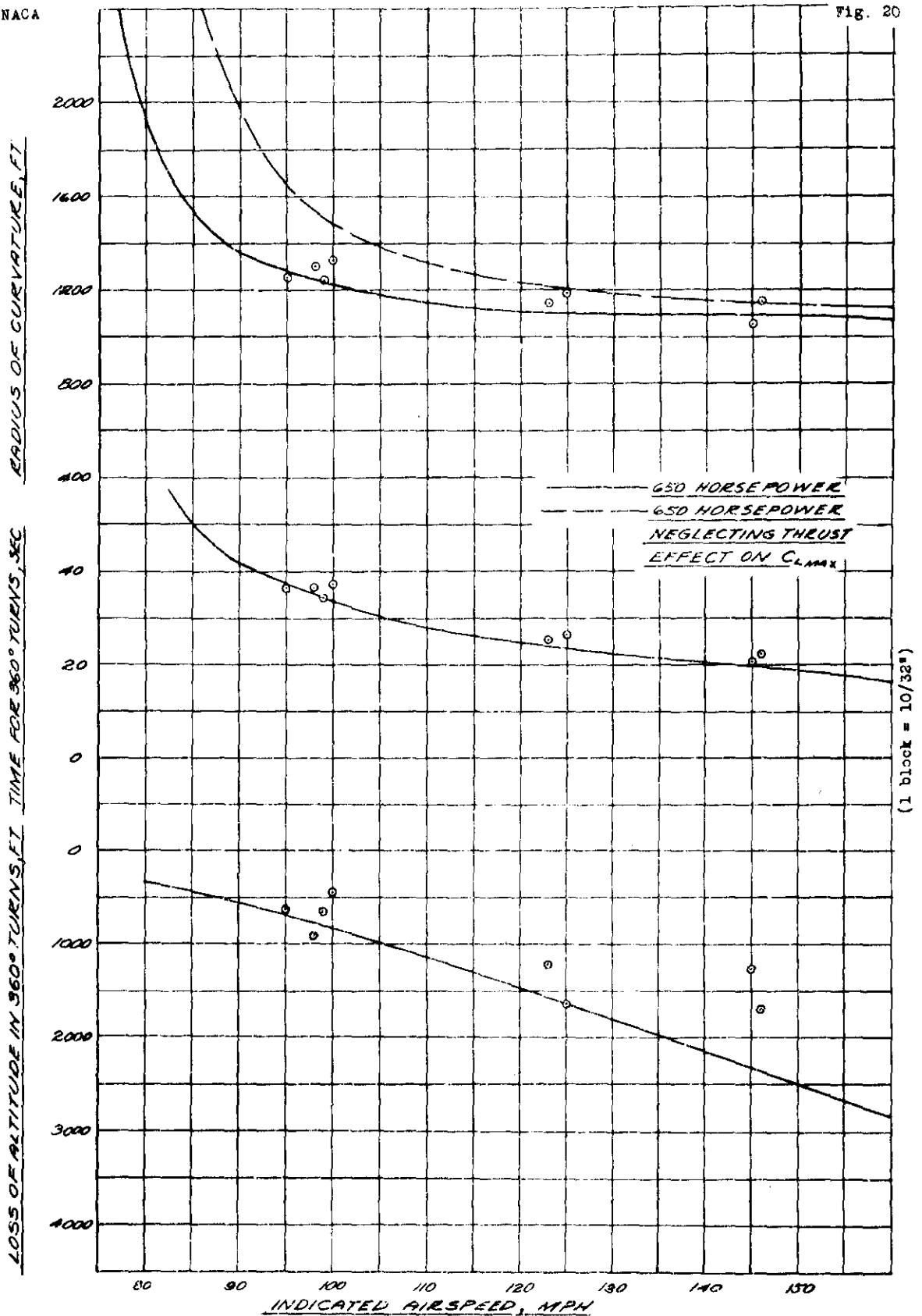
FIGURE 20.- CALCULATED AND EXPERIMENTAL DETERMINATIONS OF THE TURNING PERFORMANCE, IN STEADY TURNS, AT 27000 FEET ALTITUDE, MAXIMUM LIFT COEFFICIENT, FLAPS 22° DOWN OF A NAVY F4U-7C AIRPLANE.
