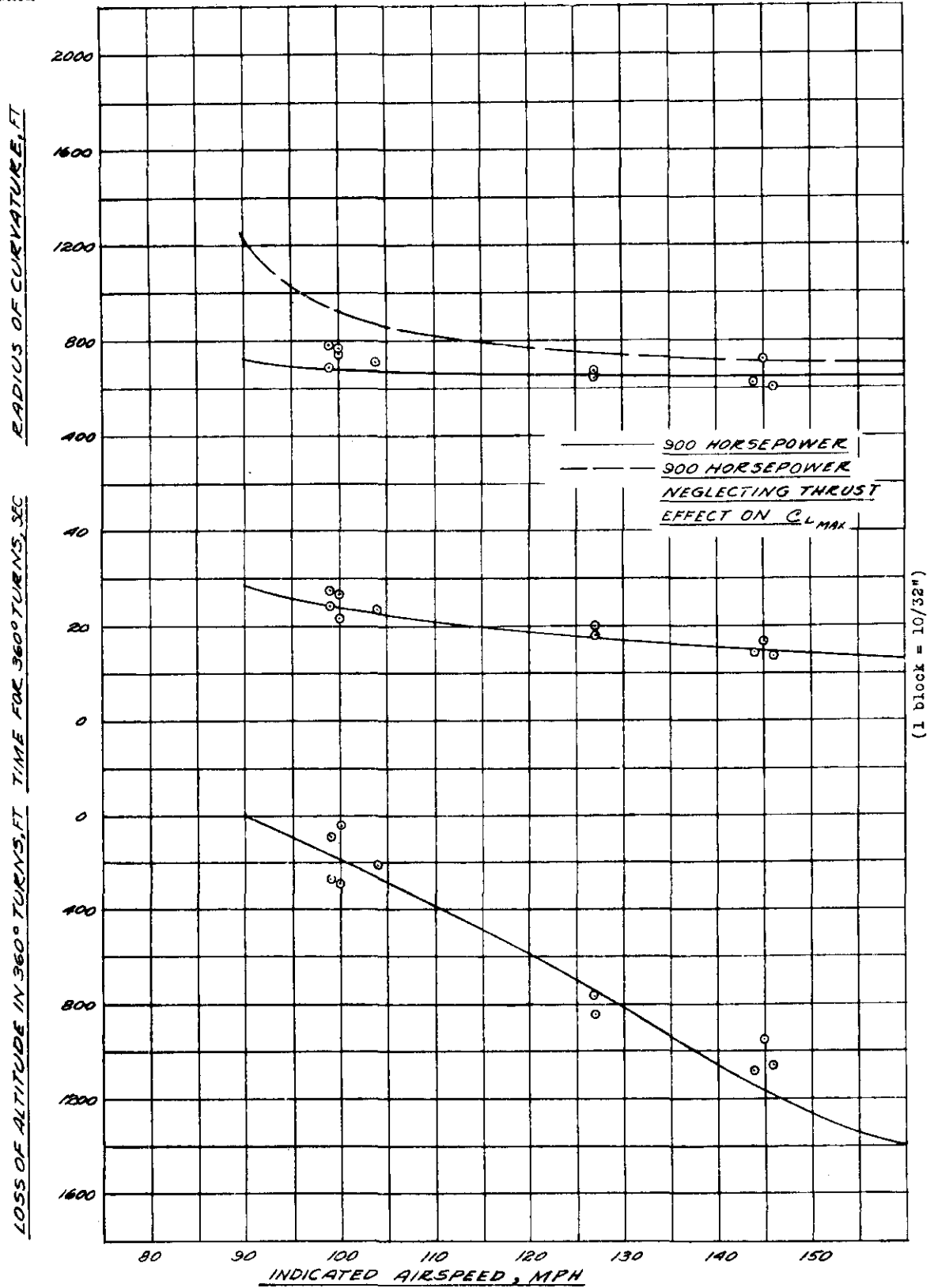
FIGURE 17. CALCULATED AND EXPERIMENTAL DETERMINATIONS OF THE TURNING PERFORMANCE, IN STEADY TURNS, AT 13000 FEET ALTITUDE, MAXIMUM LIFT COEFFICIENT, FLAPS 22° DOWN, NAVY F2A-3 AIRPLANE.
